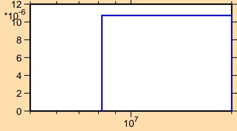
\sigma vs. E for ^{137}\text{I}(n,nt)
