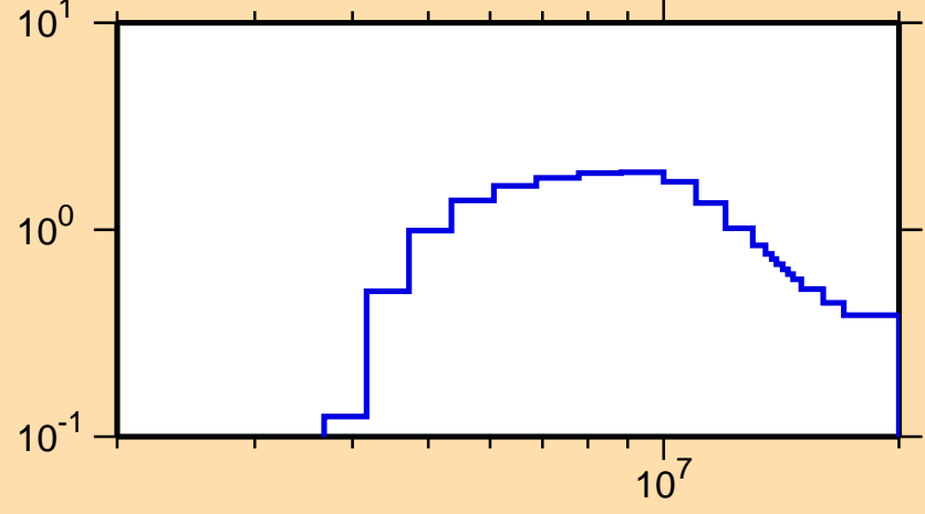
\sigma vs. E for ^{138}\text{I}(n,2n)
