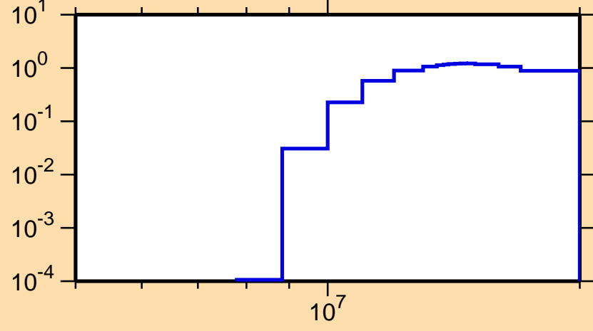
\sigma vs. E for ^{138}\text{I}(n,3n)
