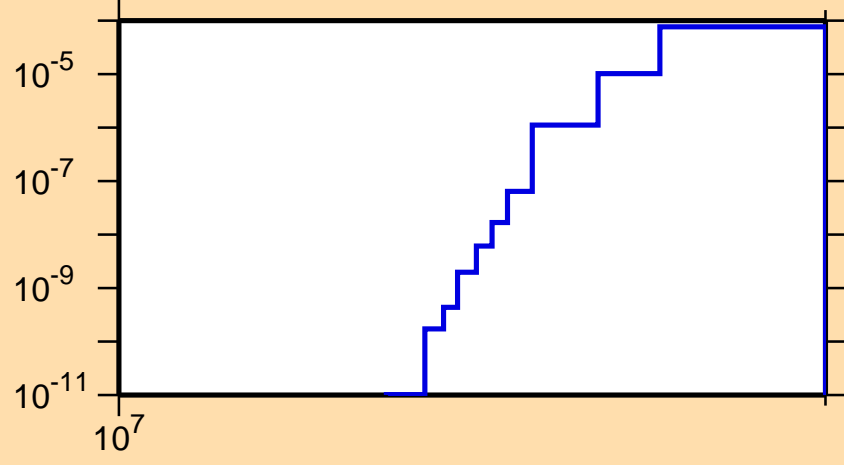
\sigma vs. E for ^{138}\text{I}(n,nd)
