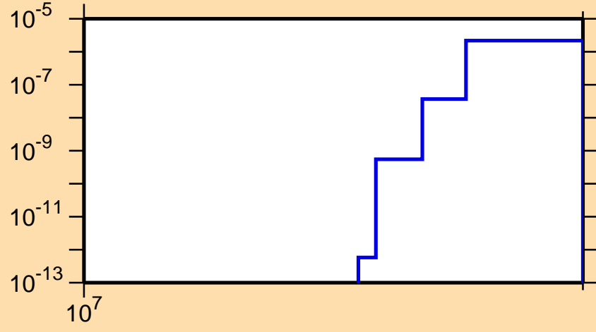
\sigma vs. E for ^{138}\text{I}(n,2np)
