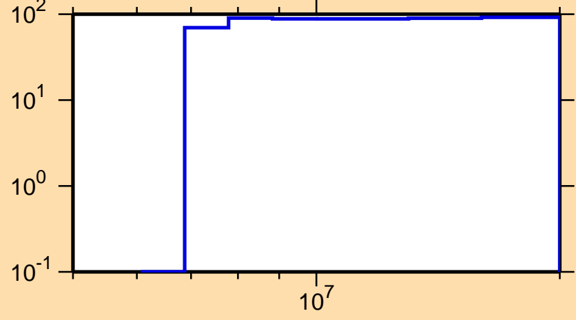
\Delta\sigma/\sigma vs. E for ^{138}\text{I}(n,p)
