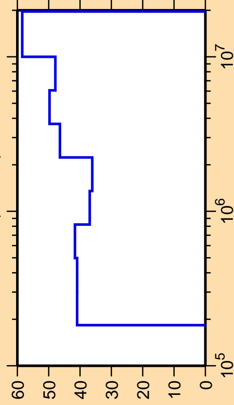
\Delta\sigma/\sigma vs. E for ^{138}\text{I}(n,\text{inel.})
