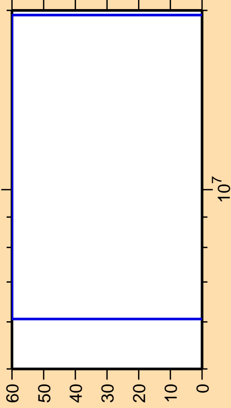
\Delta\sigma/\sigma vs. E for ^{138}\text{I}(n,p)
