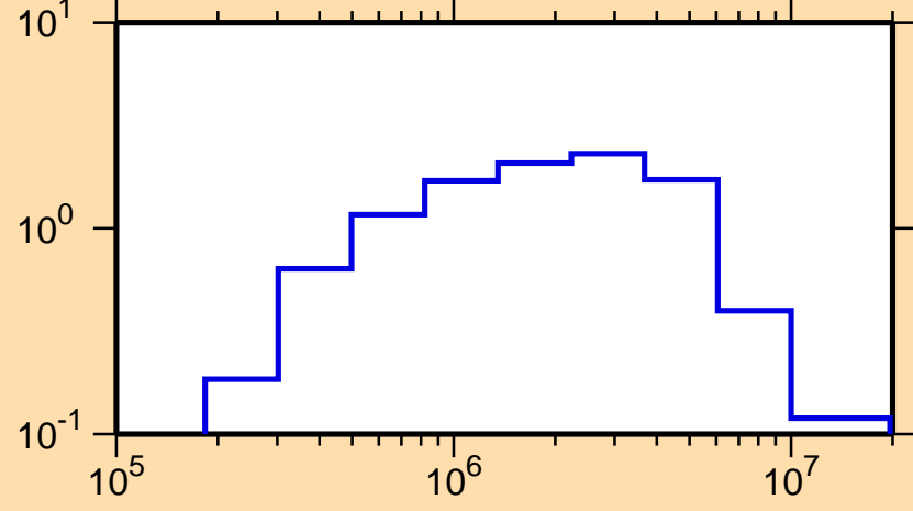
\sigma vs. E for ^{138}\text{I}(n,\text{inel.})
