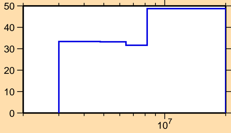
\Delta\sigma/\sigma vs. E for ^{138}\text{I}(n,2n)
