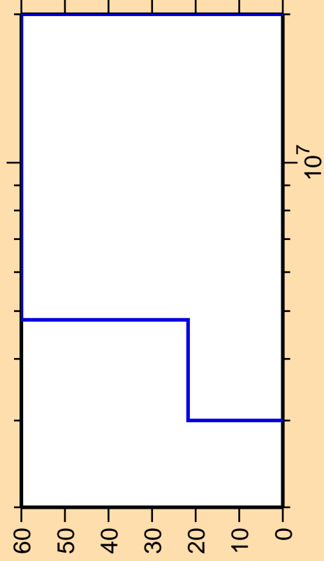
\Delta\sigma/\sigma vs. E for ^{138}\text{I}(n,n_1)
