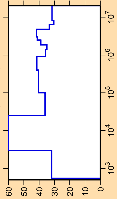
\Delta\sigma/\sigma vs. E for ^{138}\text{I}(n,\text{nonel.})
