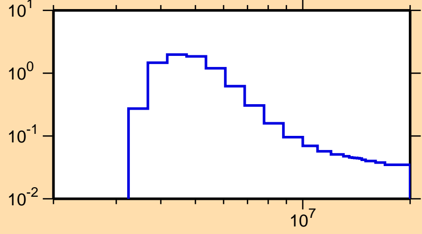
\sigma vs. E for ^{139}\text{I}(n,n\text{cont.})
