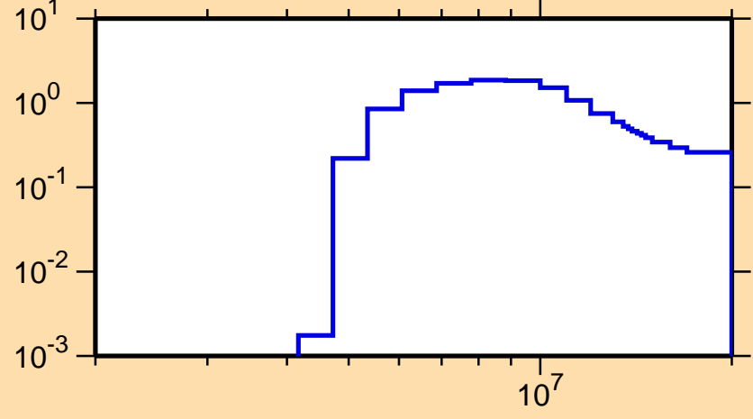
\sigma vs. E for ^{139}\text{I}(n,2n)
