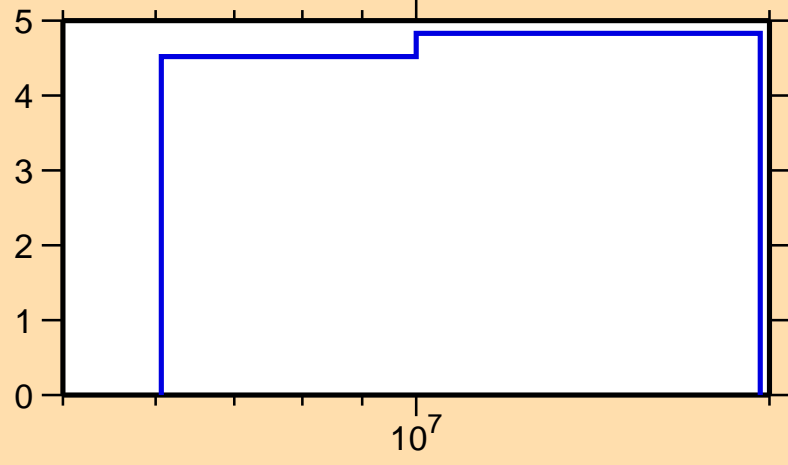
\Delta\sigma/\sigma vs. E for ^{139}\text{I}(n,tot.)
