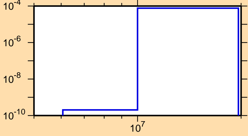
\sigma vs. E for ^{139}\text{I}(n,n\alpha)
