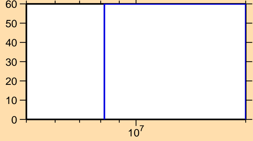
\Delta\sigma/\sigma vs. E for ^{139}\text{I}(n,p)
