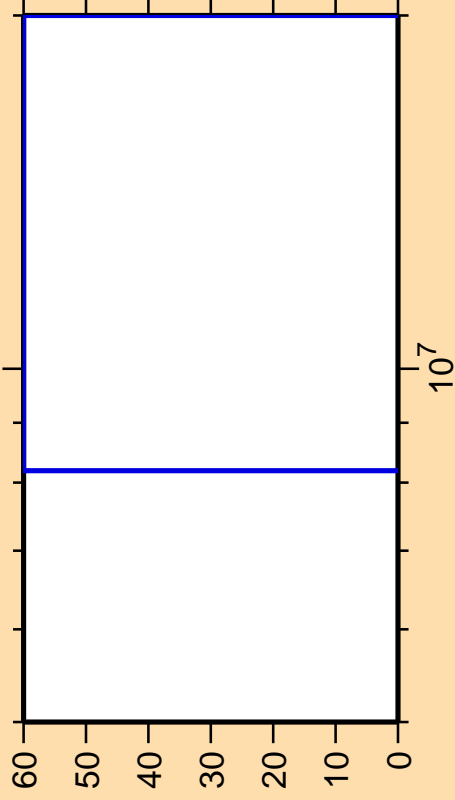
\Delta\sigma/\sigma vs. E for ^{139}\text{I}(n,\alpha)
