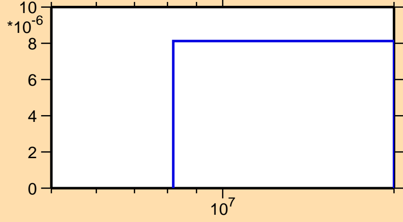
\sigma vs. E for ^{139}\text{I}(n,nt)
