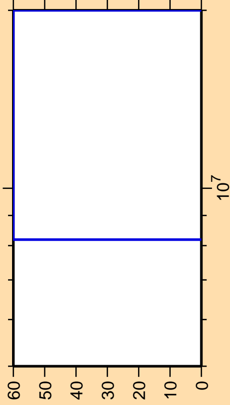
\Delta\sigma/\sigma vs. E for ^{139}\text{I}(n,p)
