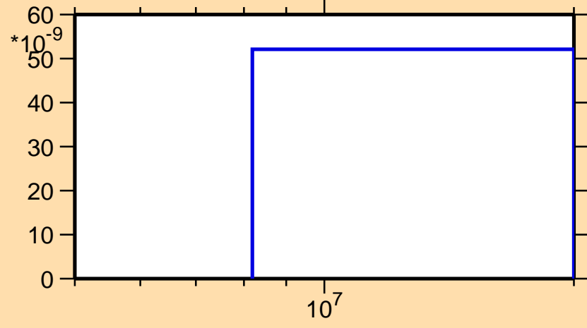
\sigma vs. E for ^{139}\text{I}(n,nd)
