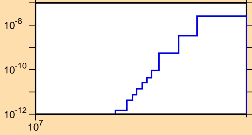
\sigma vs. E for ^{98}\text{In}(\text{mt117})
