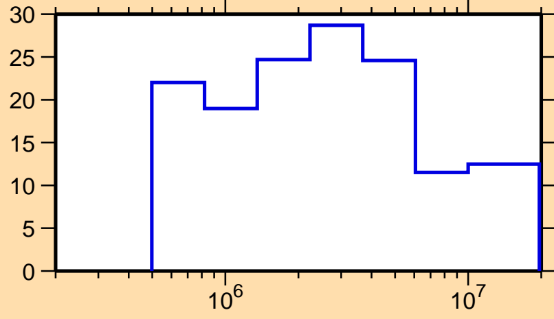
\Delta\sigma/\sigma vs. E for ^{98}\text{In}(n, el.)
