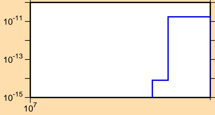
\sigma vs. E for ^{99}\text{In}(\text{mt } 34)
