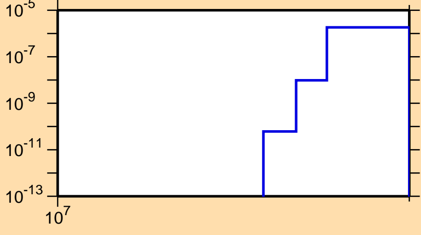
\sigma vs. E for ^{99}\text{In}(n,\text{pt})
