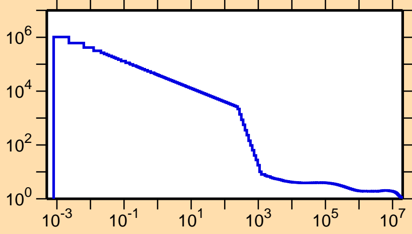
\sigma vs. E for ^{99}\text{In}(n,\text{nonel.})
