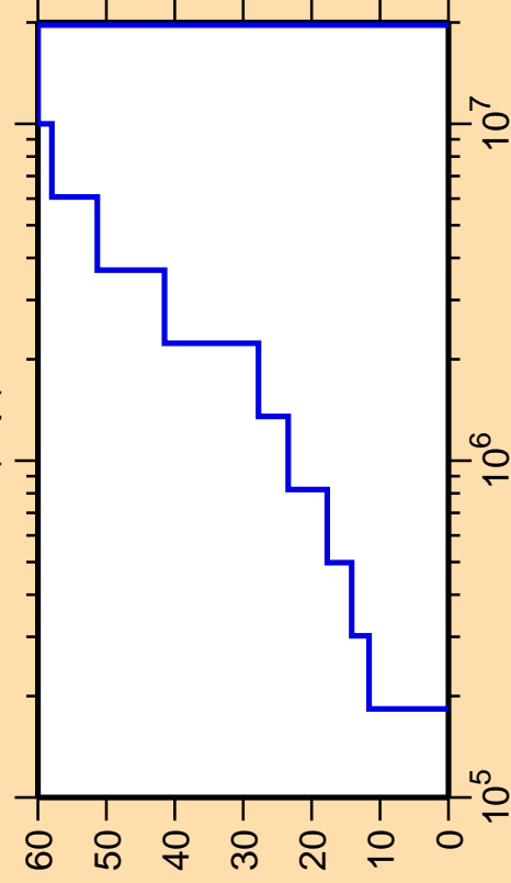
\Delta\sigma/\sigma vs. E for ^{99}\text{In}(n,p)
