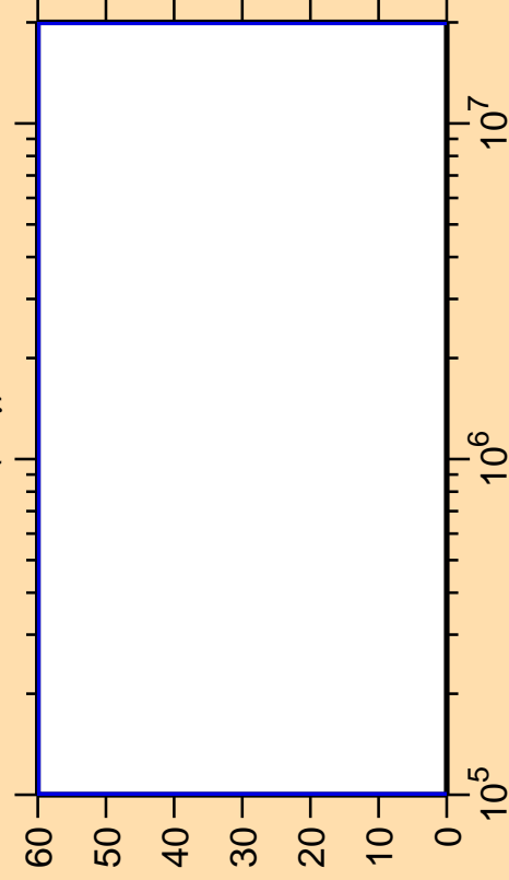
\Delta\sigma/\sigma vs. E for ^{99}\text{In}(n,\gamma)
