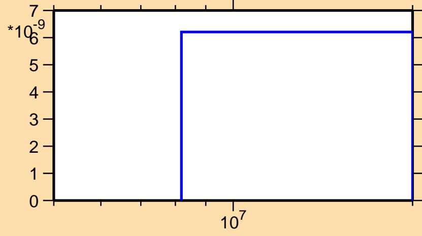
\sigma vs. E for ^{99}\text{In}(n,2np)
