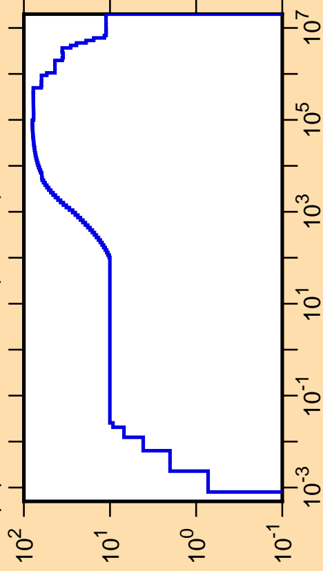
\Delta\mu/\mu vs. E for ^{100}\text{In}(\text{mt251})
