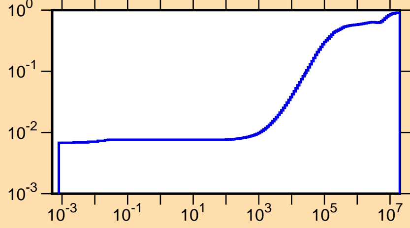
\mu vs. E for ^{100}\text{In}(\text{mt251})
