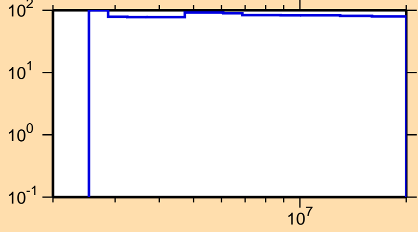
\Delta\sigma/\sigma vs. E for ^{100}\text{In}(n,n\text{cont.})
