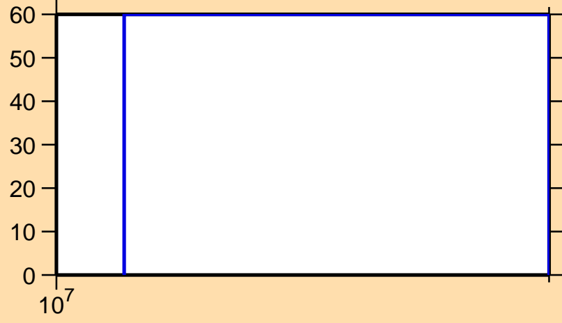
\Delta\sigma/\sigma vs. E for ^{100}\text{In}(n,\text{inel.})
