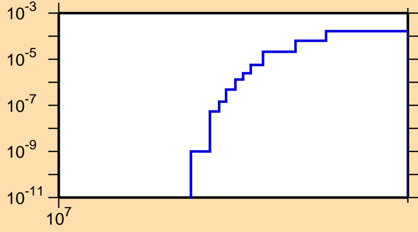
\sigma vs. E for ^{100}\text{In}(n,2np)
