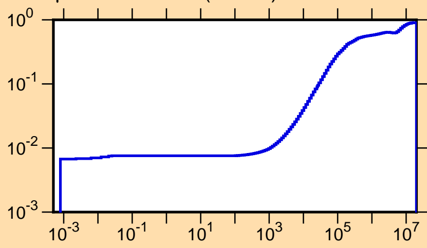
\mu vs. E for ^{101}\text{In}(\text{mt251})
