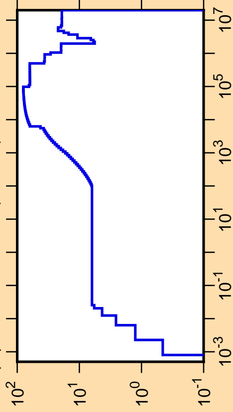
\Delta\mu/\mu vs. E for ^{101}\text{In}(\text{mt251})
