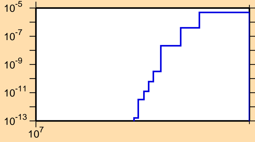
\sigma vs. E for ^{101}\text{In}(n,nd)
