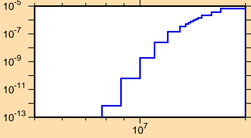
\sigma vs. E for ^{101}\text{In}(\text{mt117})
