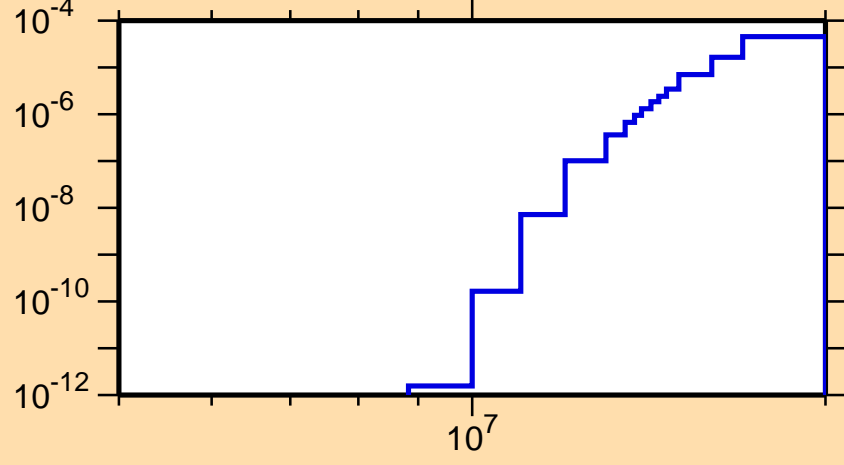
\sigma vs. E for ^{101}\text{In}(\text{mt } 45)
