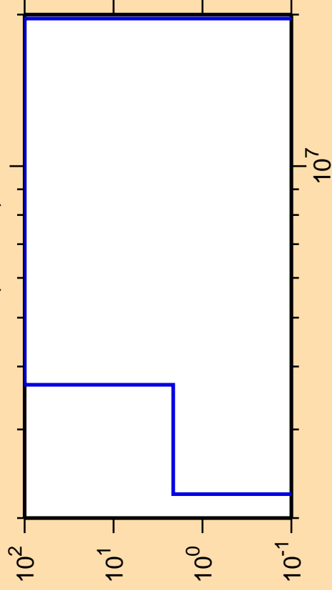
\Delta\sigma/\sigma vs. E for ^{101}\text{In}(n,\text{He3})
