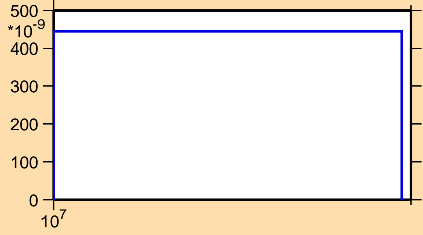
\sigma vs. E for ^{101}\text{In}(n,\text{pt})
