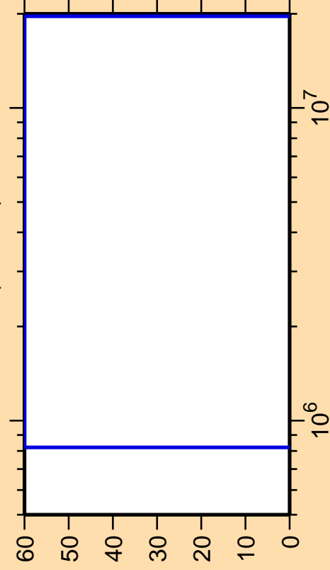
\Delta\sigma/\sigma vs. E for ^{101}\text{In}(n,\text{inel.})
