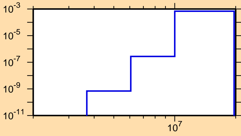
\sigma vs. E for ^{101}\text{In}(n,\text{He3})
