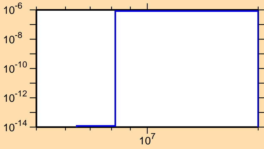
\sigma vs. E for ^{101}\text{In}(\text{mt117})
