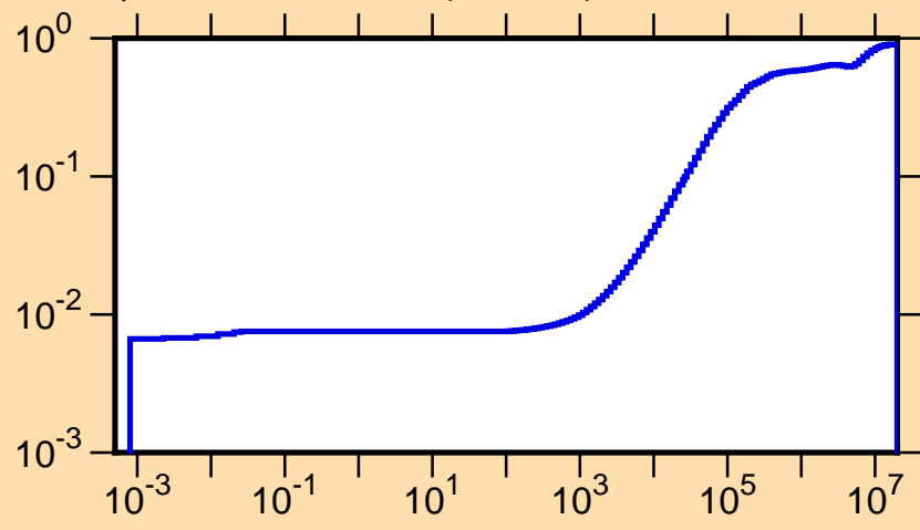
\mu vs. E for ^{102}\text{In}(\text{mt251})
