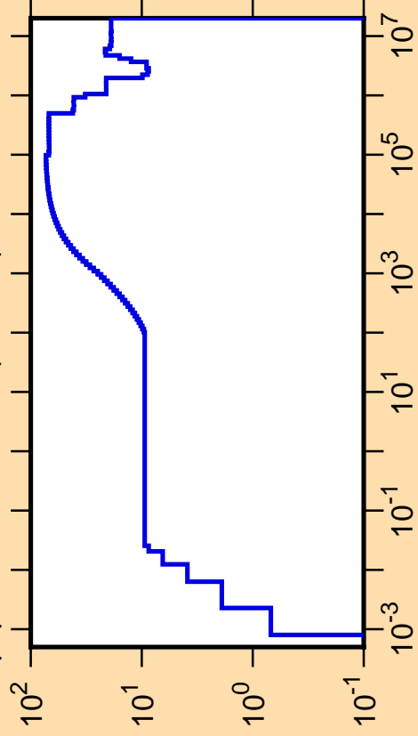
\Delta\mu/\mu vs. E for ^{102}\text{In}(\text{mt251})
