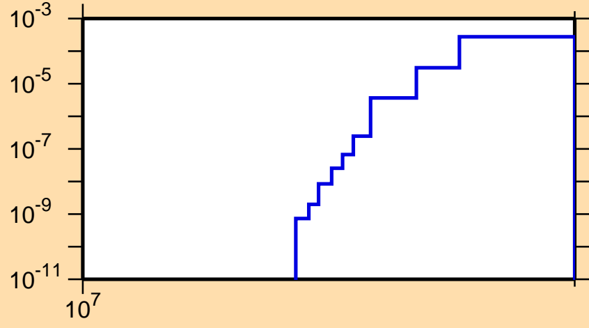
\sigma vs. E for ^{102}\text{In}(n,2np)
