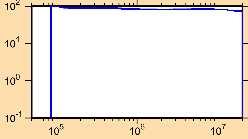
\Delta\sigma/\sigma vs. E for ^{102}\text{In}(n,\text{inel.})
