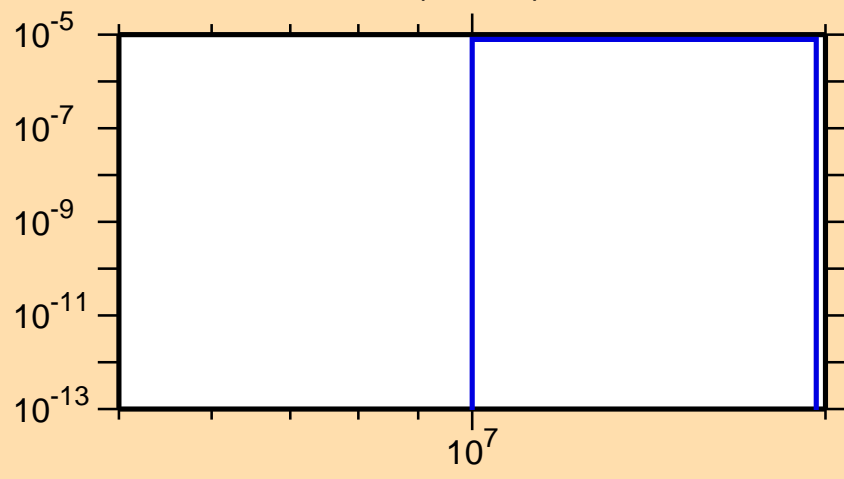
\sigma vs. E for ^{102}\text{In}(\text{mt } 45)
