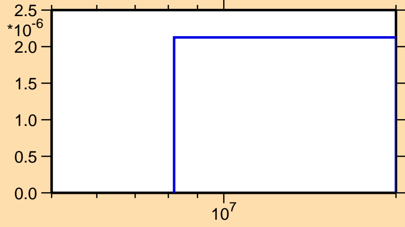
\sigma vs. E for ^{102}\text{In}(n,nd)
