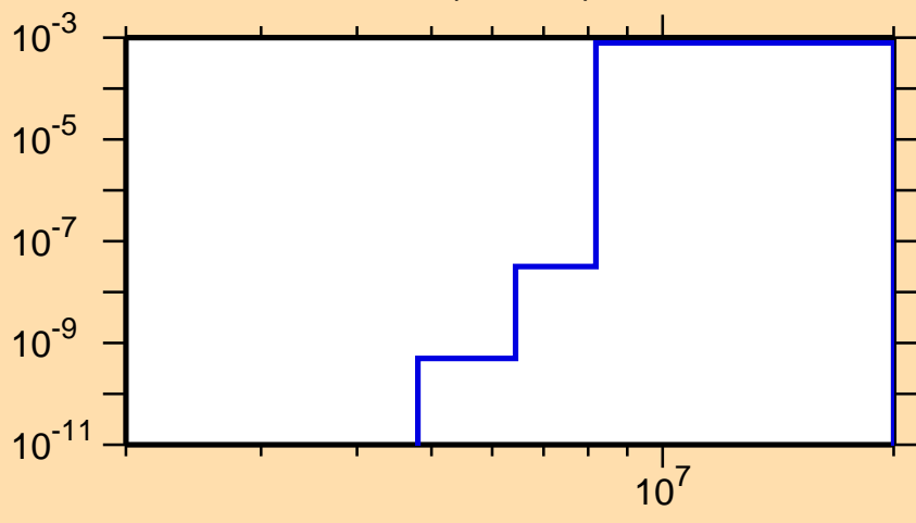
\sigma vs. E for ^{102}\text{In}(n,\text{He}3)
