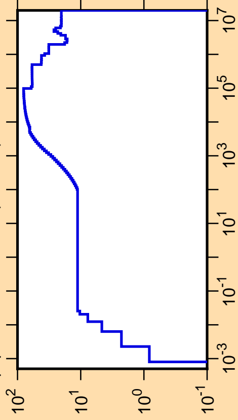
\Delta\mu/\mu vs. E for ^{103}\text{In}(\text{mt251})
