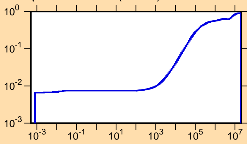
\mu vs. E for ^{103}\text{In}(\text{mt251})
