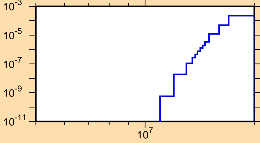
\sigma vs. E for ^{103}\text{In}(\text{mt } 45)
