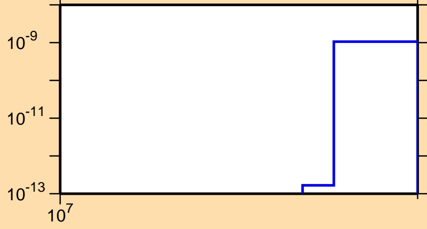
\sigma vs. E for ^{103}\text{In}(n,2n\alpha)
