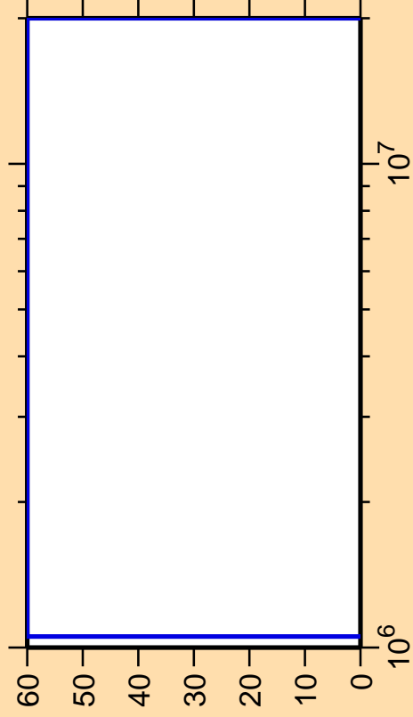
\Delta\sigma/\sigma vs. E for ^{103}\text{In}(n,n_2)
