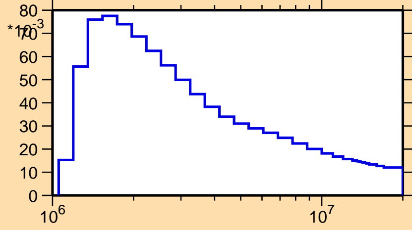
\sigma vs. E for ^{103}\text{In}(n,n_2)
