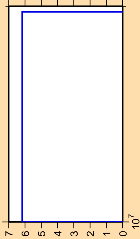
\Delta\sigma/\sigma vs. E for ^{103}\text{In}(n,2n\alpha)
