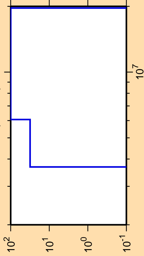
\Delta\sigma/\sigma vs. E for ^{103}\text{In}(n,\text{He3})
