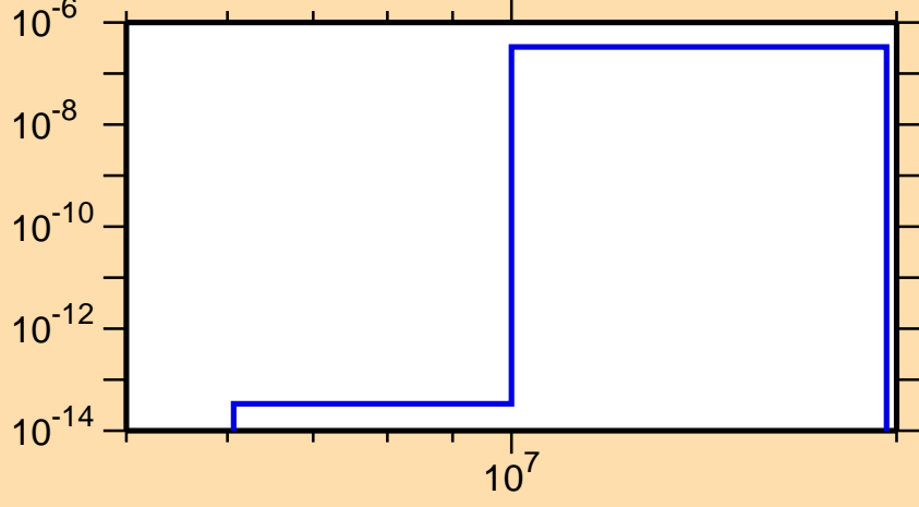
\sigma vs. E for ^{103}\text{In}(\text{mt117})
