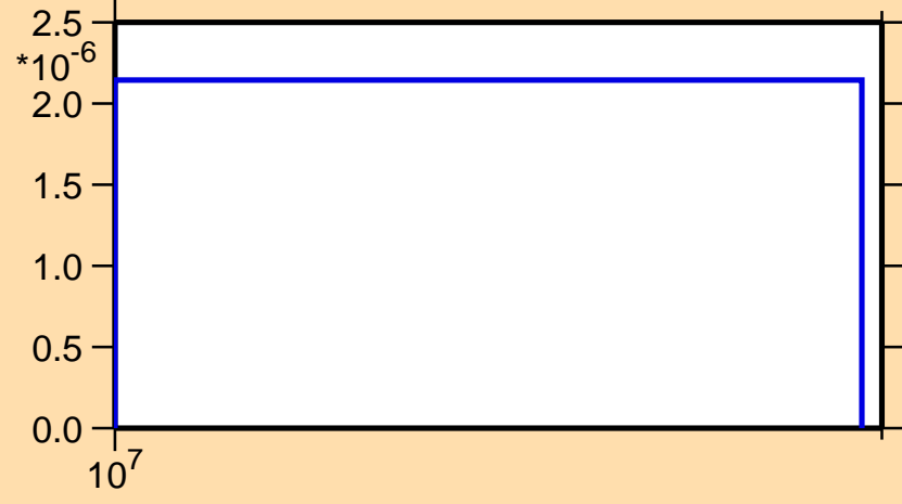
\sigma vs. E for ^{103}\text{In}(n,2np)
