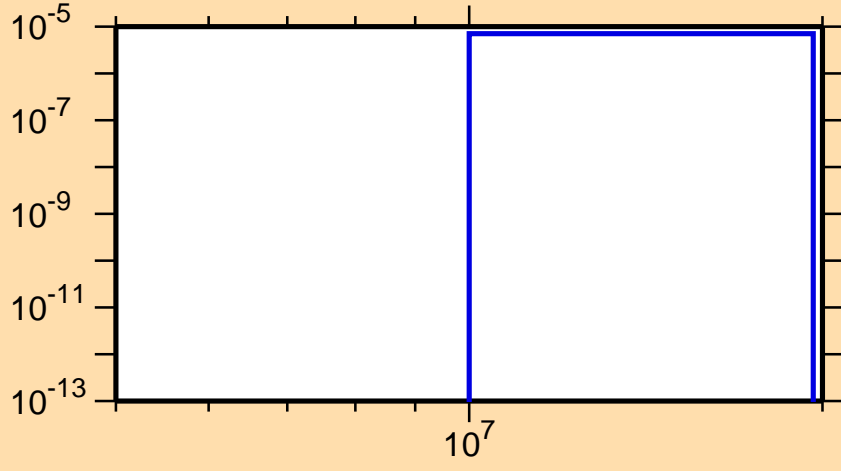
\sigma vs. E for ^{103}\text{In}(\text{mt } 45)
