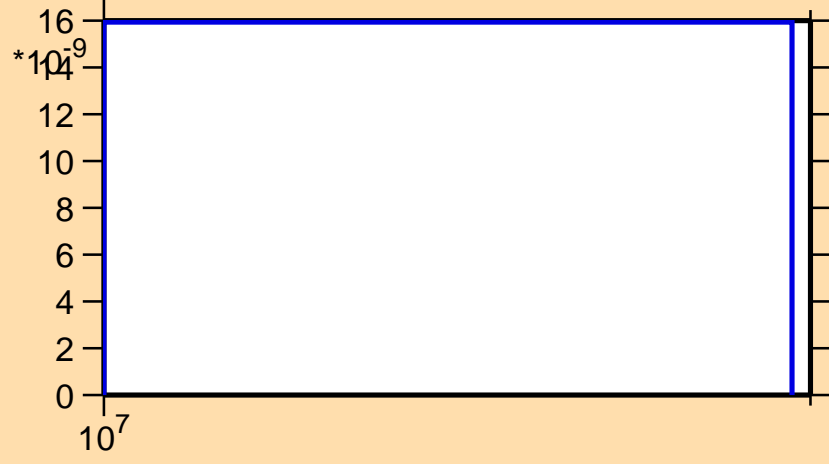
\sigma vs. E for ^{103}\text{In}(n,\text{pt})
