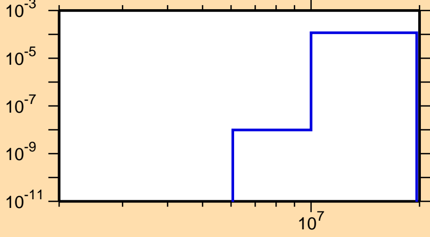
\sigma vs. E for ^{103}\text{In}(n,\text{He3})
