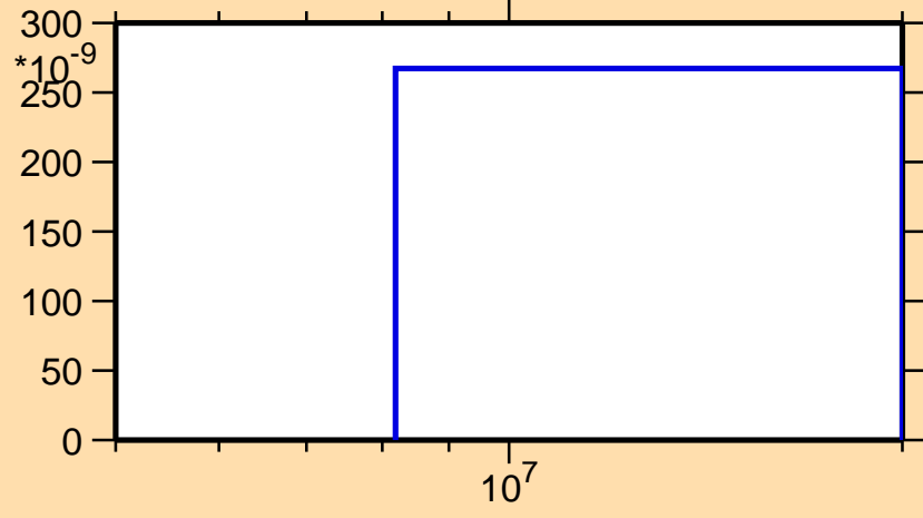
\sigma vs. E for ^{103}\text{In}(\text{mt117})
