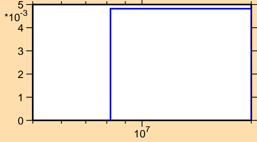
\sigma vs. E for ^{103}\text{In}(n,2n)
