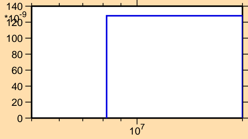
\sigma vs. E for ^{103}\text{In}(n,nd)
