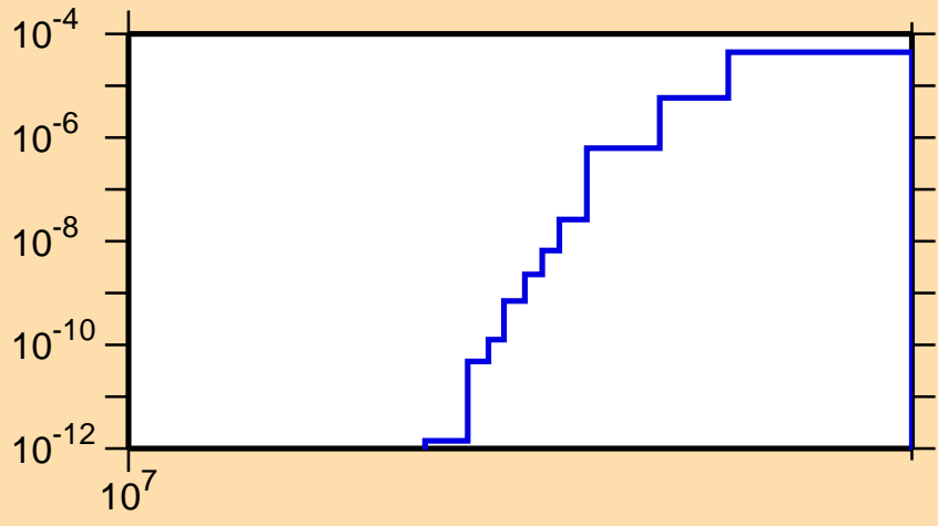
\sigma vs. E for ^{103}\text{In}(n,nd)
