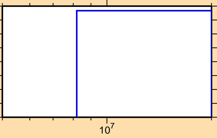
\sigma vs. E for ^{103}\text{In}(\text{mt } 45)
