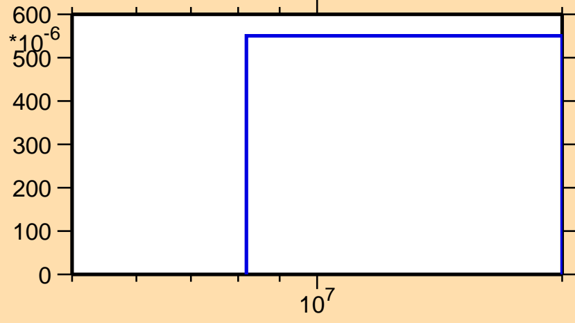
\sigma vs. E for ^{103}\text{In}(n,pd)
