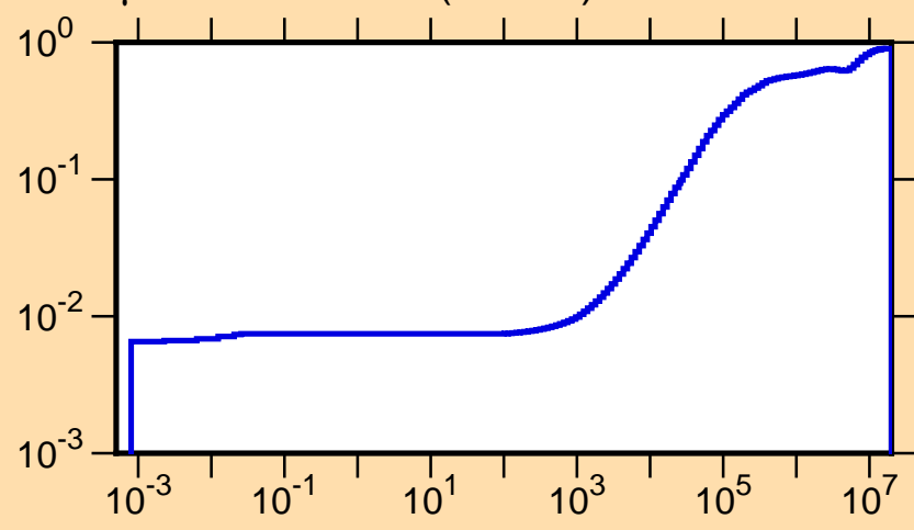
\mu vs. E for ^{104}\text{In}(\text{mt251})
