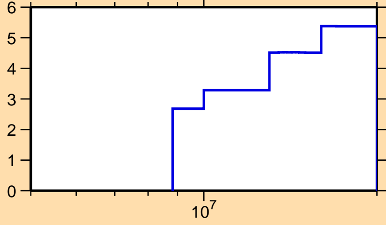
\Delta\sigma/\sigma vs. E for ^{104}\text{In}(n,\text{tot.})
