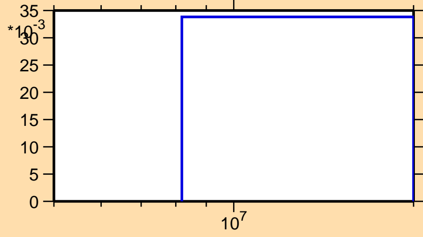
\sigma vs. E for ^{104}\text{In}(n,2n)
