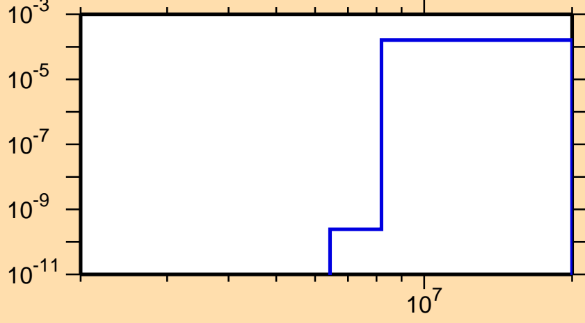
\sigma vs. E for ^{104}\text{In}(n,\text{He3})
