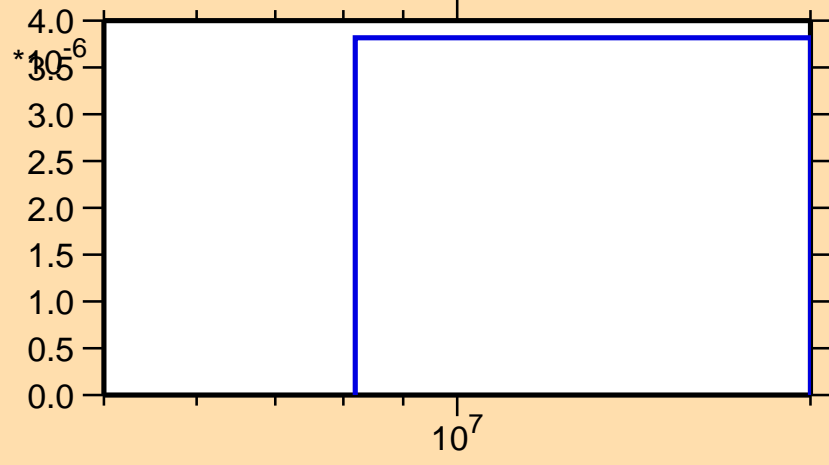
\sigma vs. E for ^{104}\text{In}(\text{mt } 45)
