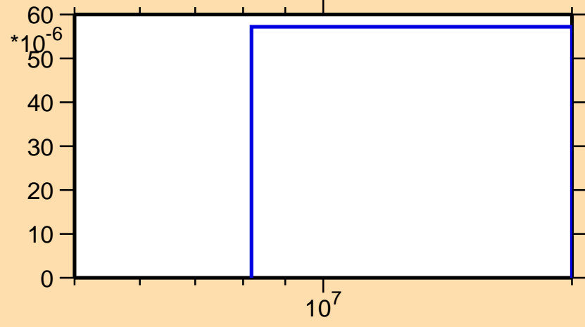
\sigma vs. E for ^{104}\text{In}(n,\text{pd})
