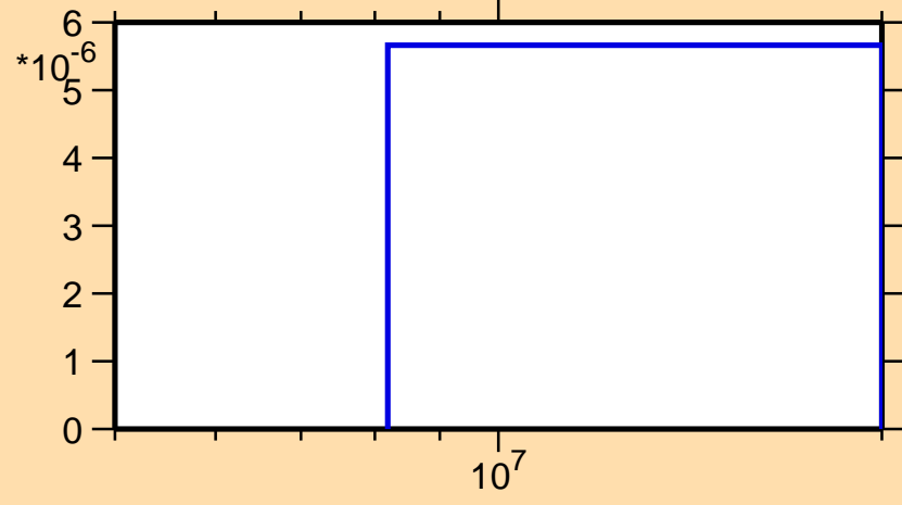
\sigma vs. E for ^{104}\text{In}(n,\text{nd})
