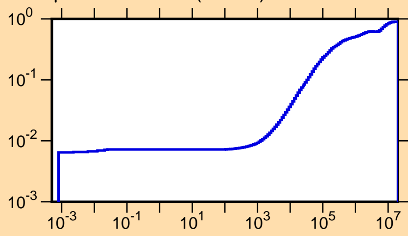
\mu vs. E for ^{105}\text{In}(\text{mt251})
