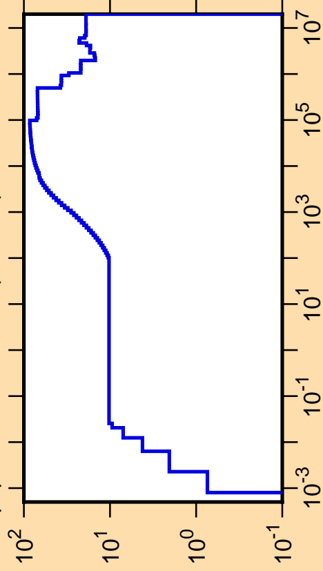
\Delta\mu/\mu vs. E for ^{105}\text{In}(\text{mt251})
