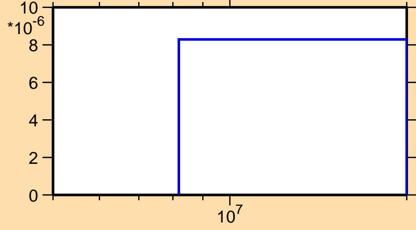
\sigma vs. E for ^{105}\text{In}(n,\text{pd})
