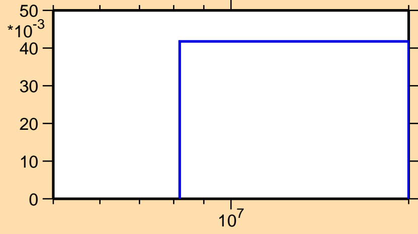
\sigma vs. E for ^{105}\text{In}(n,2n)
