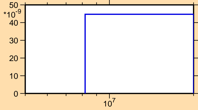
\sigma vs. E for ^{105}\text{In}(\text{mt117})
