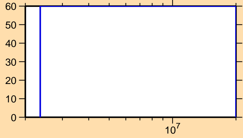
\Delta\sigma/\sigma vs. E for ^{105}\text{In}(n,n\text{cont.})
