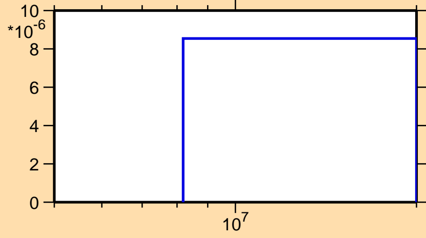
\sigma vs. E for ^{105}\text{In}(n,2np)
