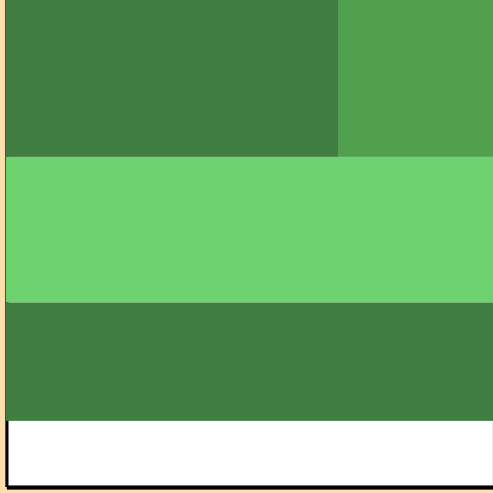
\Delta\sigma/\sigma vs. E for ^{105}\text{In}(n,\text{tot.})
