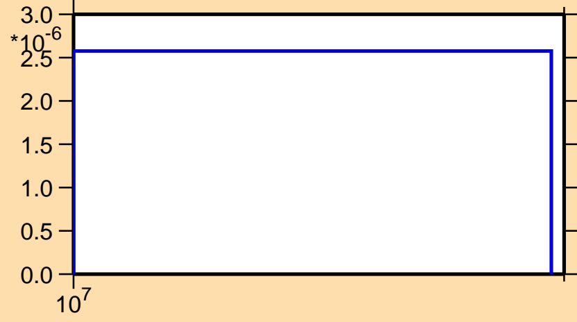
\sigma vs. E for ^{105}\text{In}(n,nd)
