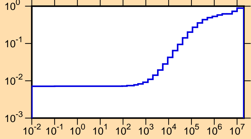
\mu vs. E for ^{106}\text{In}(\text{mt251})
