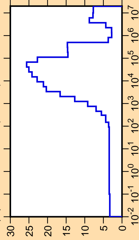
\Delta\mu/\mu vs. E for ^{106}\text{In}(\text{mt251})
