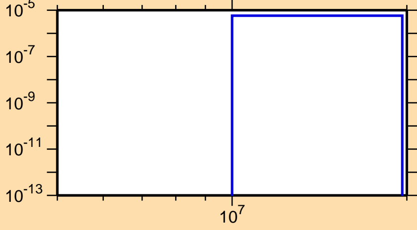
\sigma vs. E for ^{106}\text{In}(n,nd)
