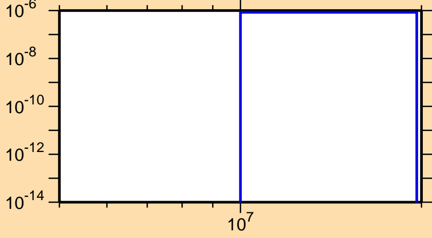
\sigma vs. E for ^{106}\text{In}(n,\text{pd})
