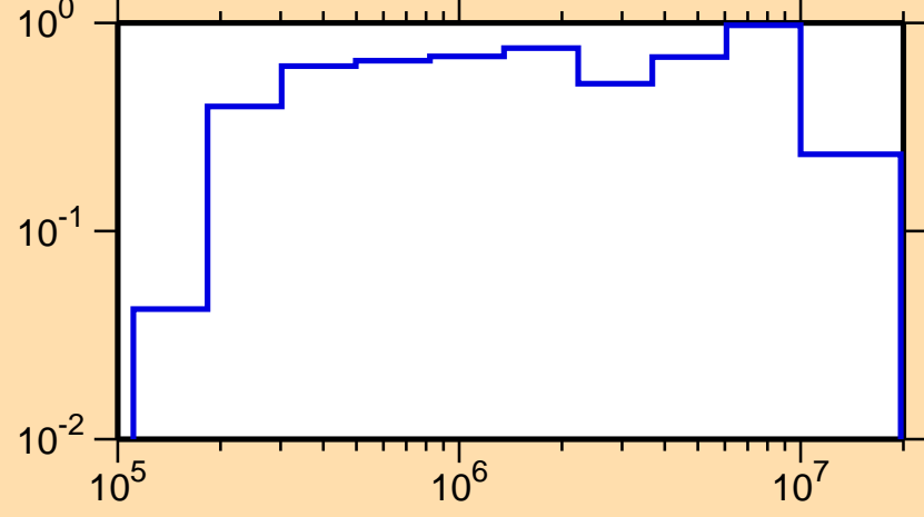
\sigma vs. E for ^{106}\text{In}(n,\text{inel.})
