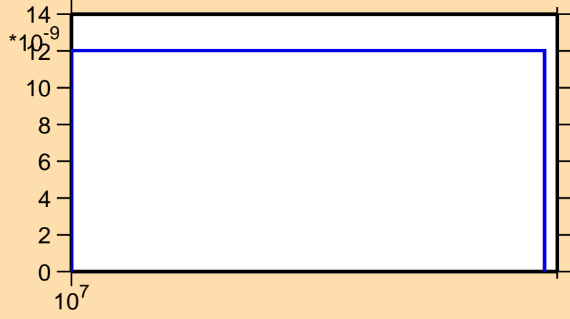
\sigma vs. E for ^{106}\text{In}(n,\text{pt})
