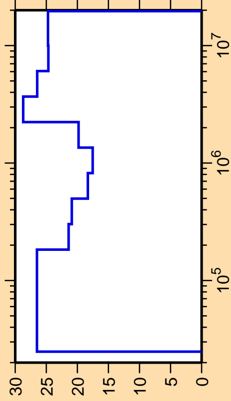
\Delta\sigma/\sigma vs. E for ^{106}\text{In}(n,\text{inel.})
