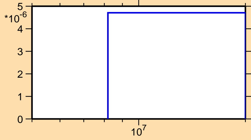
\sigma vs. E for ^{106}\text{In}(n,\text{nd})
