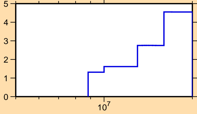
\Delta\sigma/\sigma vs. E for ^{106}\text{In}(n,\text{tot.})
