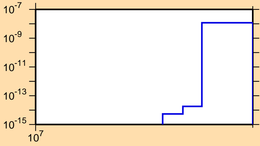
\sigma vs. E for ^{106}\text{In}(n,nt)
