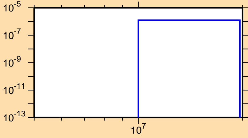
\sigma vs. E for ^{106}\text{In}(n,\text{pd})
