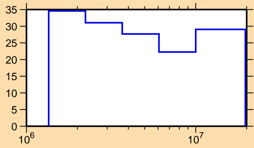
\Delta\sigma/\sigma vs. E for ^{106}\text{In}(n,ncont.)
