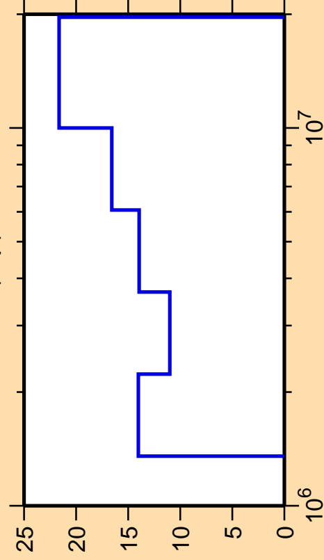
\Delta\sigma/\sigma vs. E for ^{106}\text{In}(n,p)
