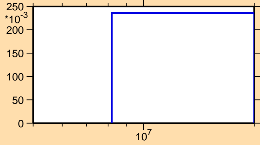
\sigma vs. E for ^{106}\text{In}(n,2n)
