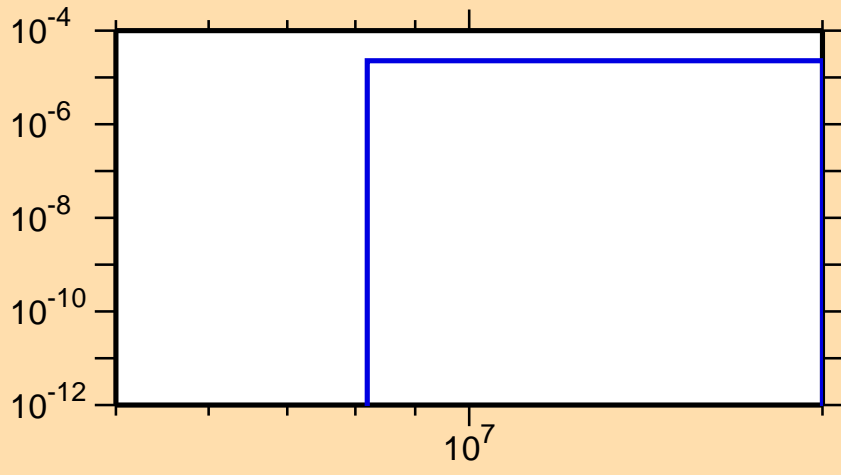
\sigma vs. E for ^{106}\text{In}(n,\text{He3})
