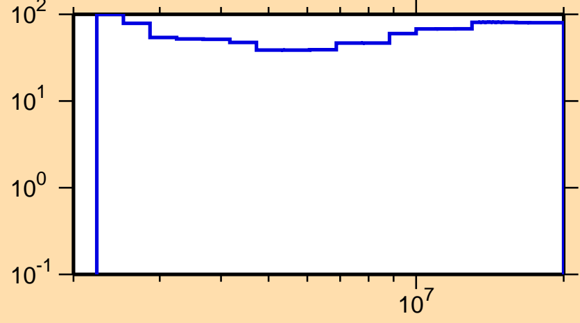
\Delta\sigma/\sigma vs. E for ^{107}\text{In}(n,n\text{cont.})
