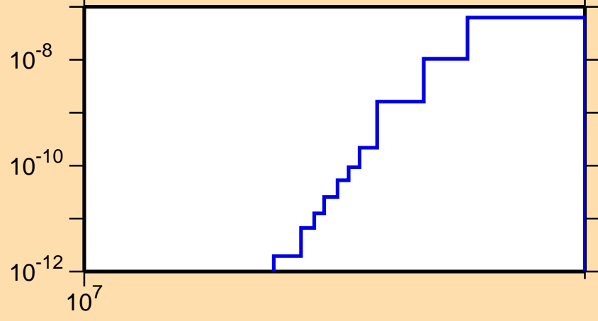
\sigma vs. E for ^{107}\text{In}(\text{mt117})
