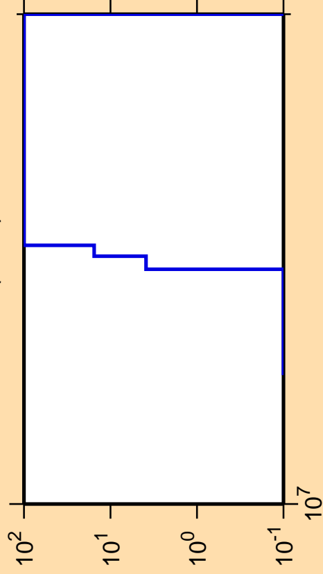
\Delta\sigma/\sigma vs. E for ^{107}\text{In}(n,nd)
