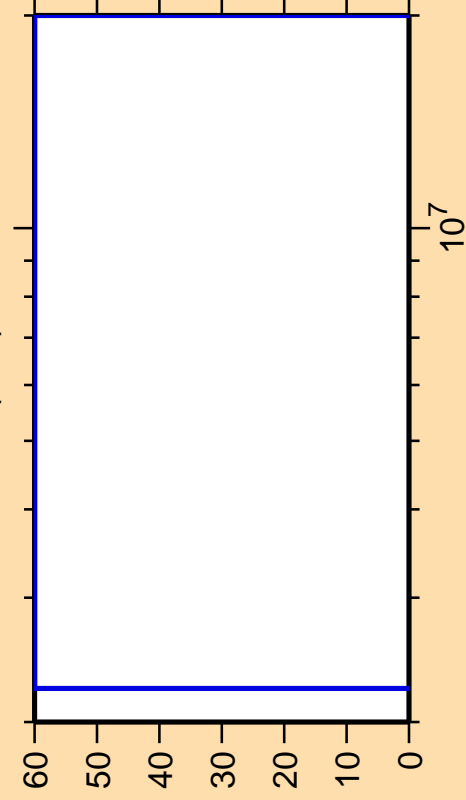
\Delta\sigma/\sigma vs. E for ^{107}\text{In}(n,\alpha)
