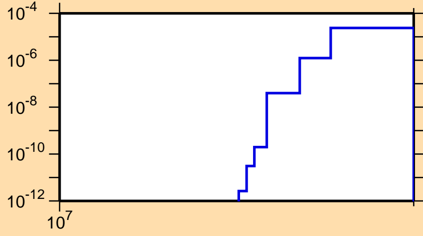
\sigma vs. E for ^{107}\text{In}(n,nd)
