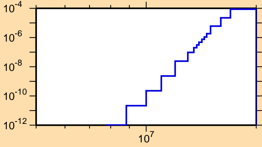
\sigma vs. E for ^{107}\text{In}(n,\text{He3})
