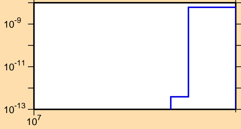
\sigma vs. E for ^{107}\text{In}(n,\text{pt})
