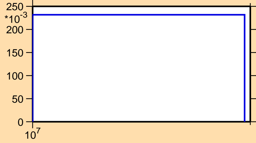
\sigma vs. E for ^{107}\text{In}(n,2n)
