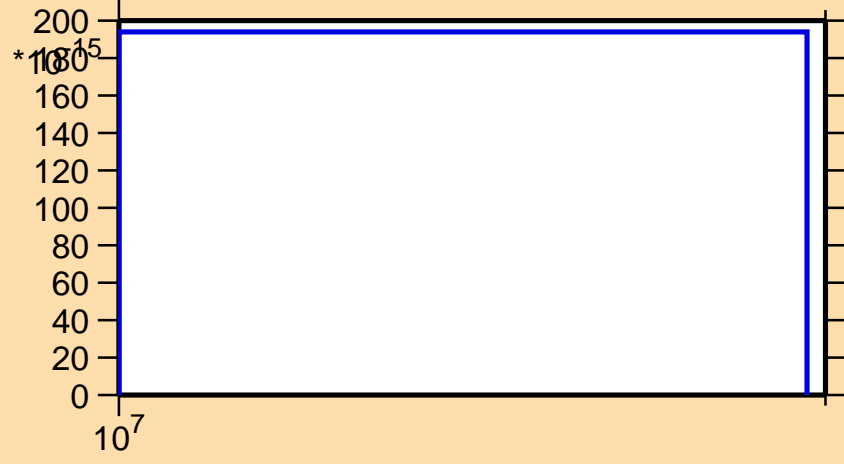
\sigma vs. E for ^{107}\text{In}(\text{mt } 34)
