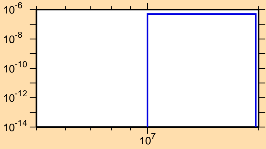
\sigma vs. E for ^{107}\text{In}(n,\text{pd})
