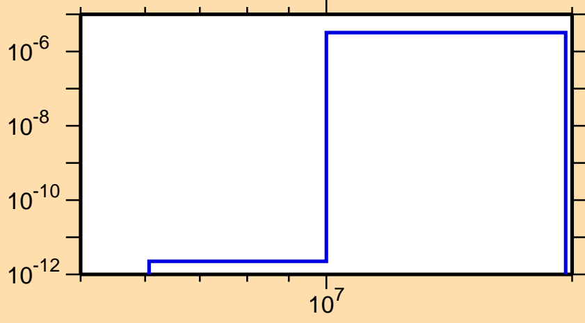
\sigma vs. E for ^{107}\text{In}(n,\text{He3})
