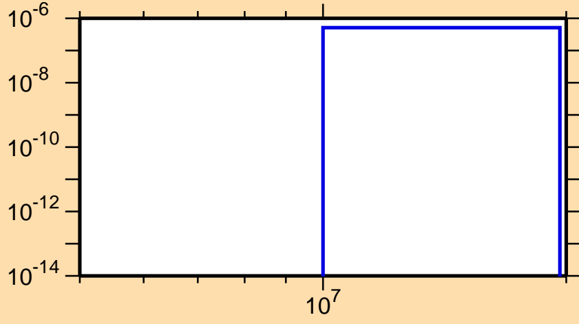
\sigma vs. E for ^{107}\text{In}(\text{mt } 45)
