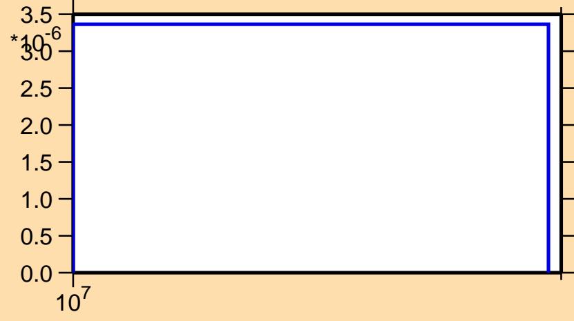
\sigma vs. E for ^{108}\text{In}(n,\text{nd})
