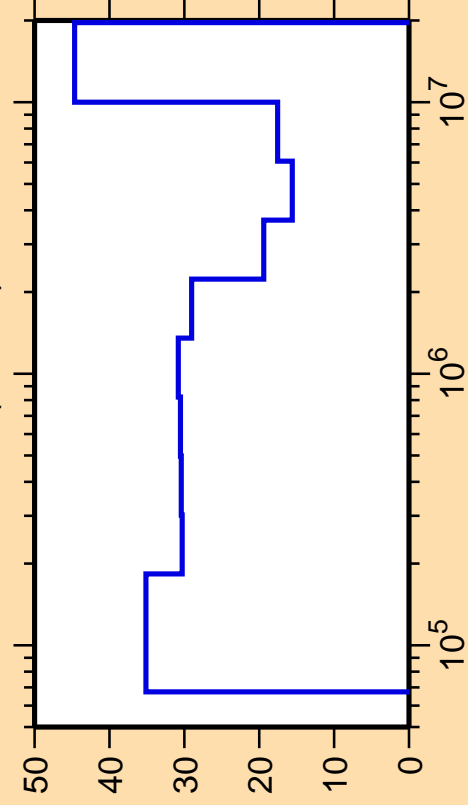
\Delta\sigma/\sigma vs. E for ^{108}\text{In}(n,\text{inel.})
