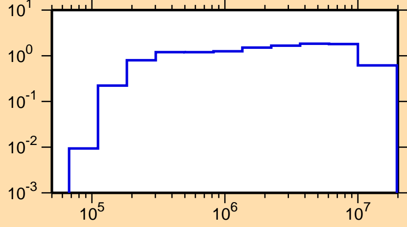
\sigma vs. E for ^{108}\text{In}(n,\text{inel.})
