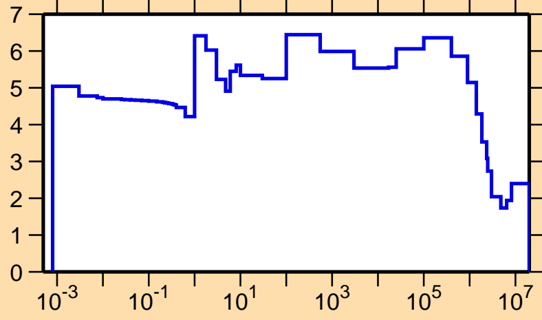
\sigma vs. E for ^{108}\text{In}(n,\text{el.})
