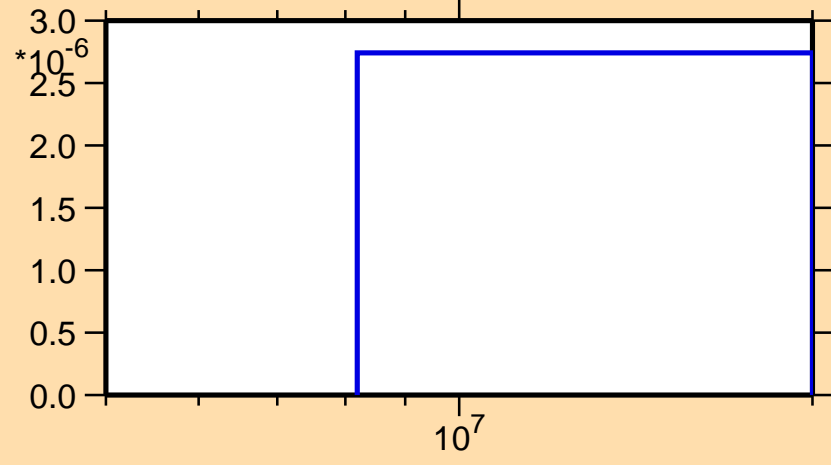
\sigma vs. E for ^{108}\text{In}(n,nd)
