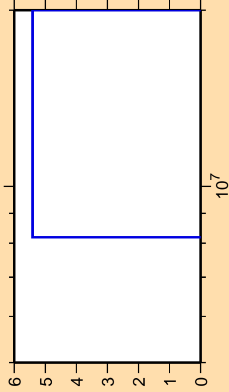
\Delta\sigma/\sigma vs. E for ^{108}\text{In}(\text{mt } 34)
