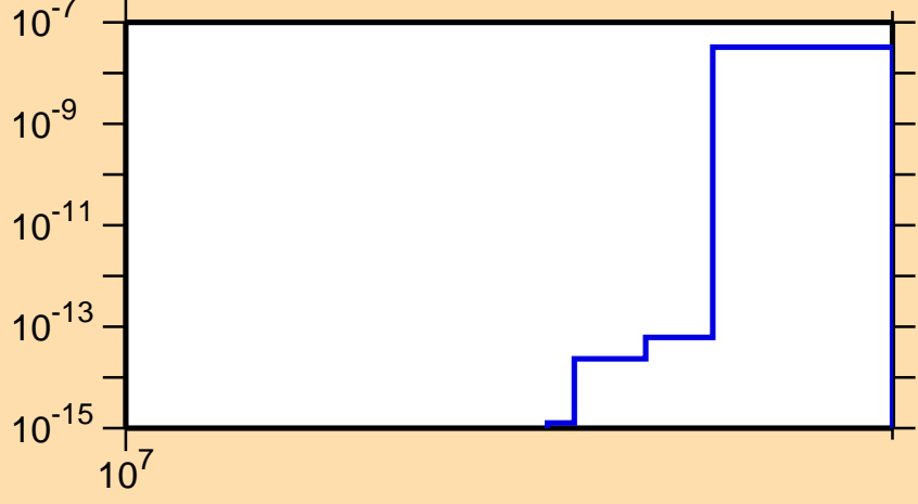
\sigma vs. E for ^{108}\text{In}(n,nt)
