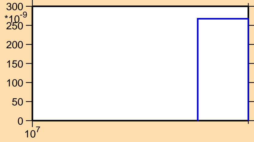
\sigma vs. E for ^{108}\text{In}(n,3n)
