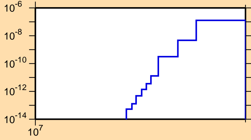
\sigma vs. E for ^{108}\text{In}(mt\ 45)
