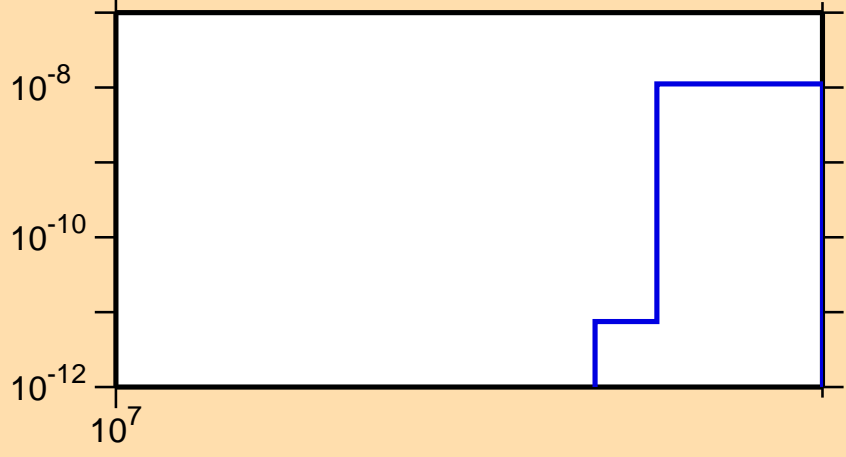
\sigma vs. E for ^{108}\text{In}(n,\text{pt})
