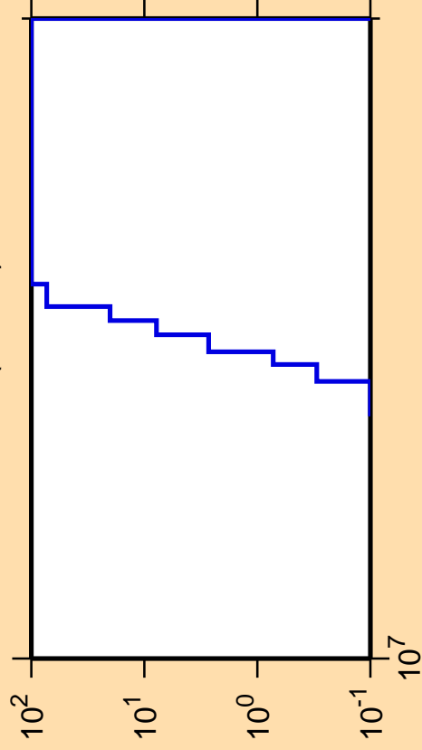
\Delta\sigma/\sigma vs. E for ^{108}\text{In}(mt\ 45)
