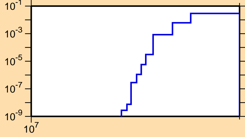
\sigma vs. E for ^{108}\text{In}(n,2np)
