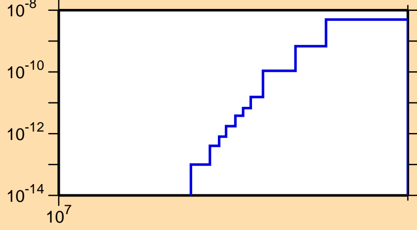
\sigma vs. E for ^{108}\text{In}(\text{mt117})
