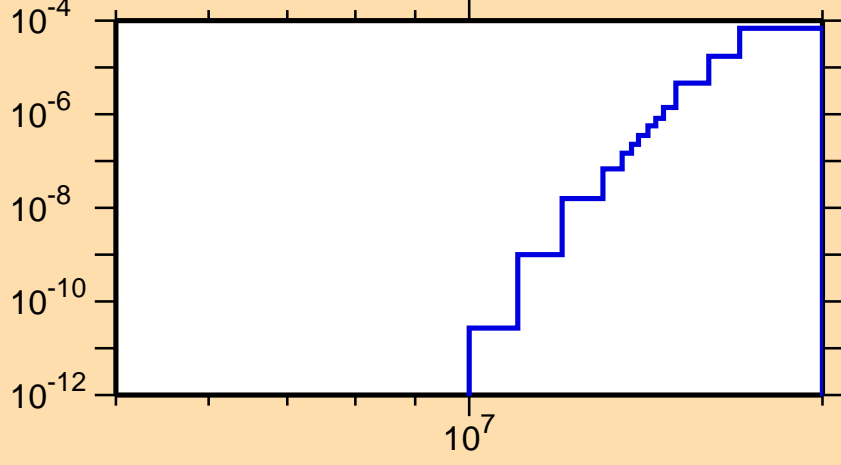
\sigma vs. E for ^{108}\text{In}(n,\text{He3})
