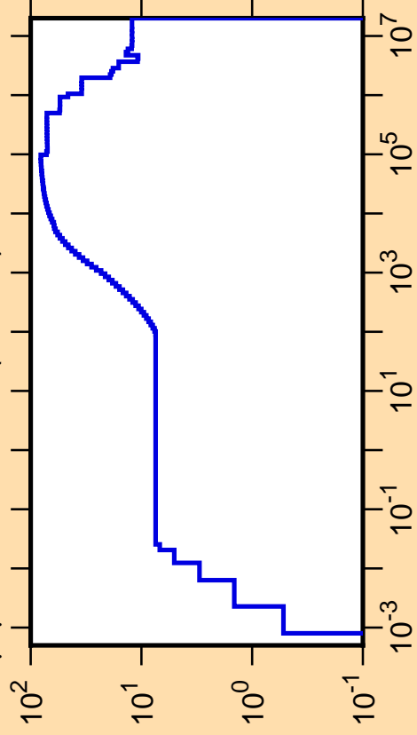
\Delta\mu/\mu vs. E for ^{109}\text{In}(\text{mt251})
