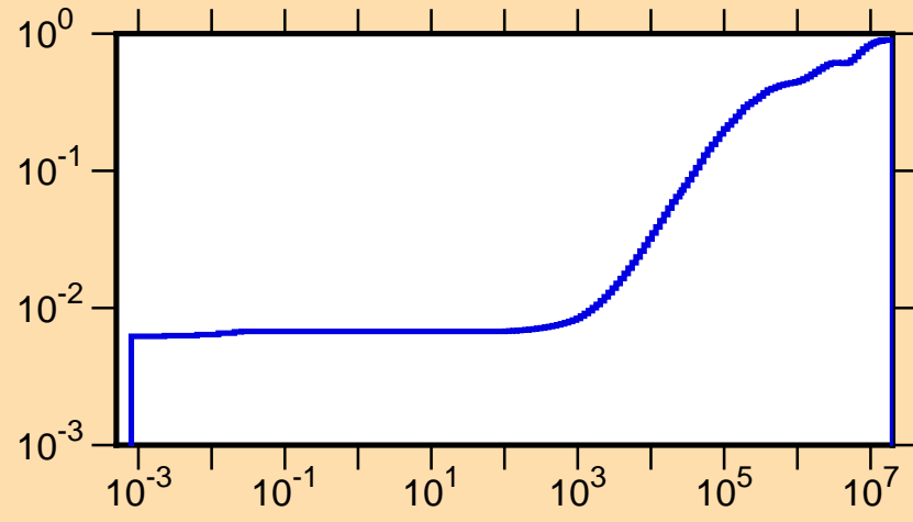
\mu vs. E for ^{109}\text{In}(\text{mt251})
