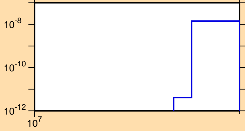
\sigma vs. E for ^{109}\text{In}(n,2n\alpha)
