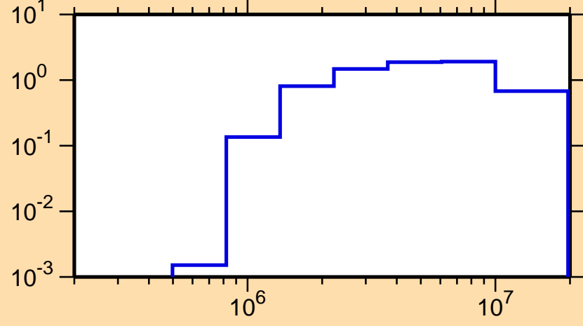
\sigma vs. E for ^{109}\text{In}(n,\text{inel.})
