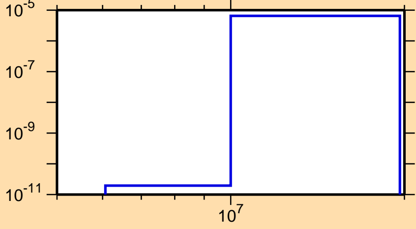
\sigma vs. E for ^{109}\text{In}(n,p\alpha)
