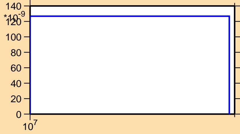
\sigma vs. E for ^{109}\text{In}(n,nd)
