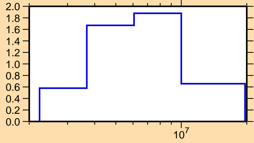
\sigma vs. E for ^{109}\text{In}(n,n\text{cont.})
