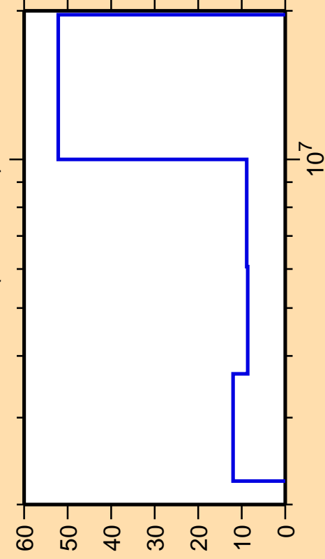
\Delta\sigma/\sigma vs. E for ^{109}\text{In}(n,\text{ncont.})
